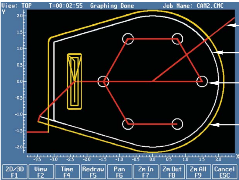
Thread Milling
